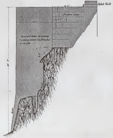
ELEVATION OF THE TOWERS OF OPHEL FROM THE NORTH.
